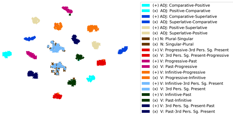
Figure 4: t-SNE visualization of all demo relation pairs from English validation set embedded by the relation encoder. Each point is colored by the relation type that it represents.
